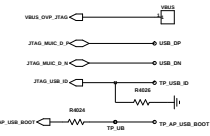
IROM BOOT
