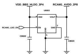
RCAM1_AVDD
