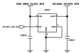
RCAM1_AFVDD
